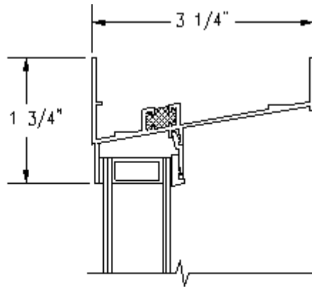
① SINGLE HUNG HEAD
