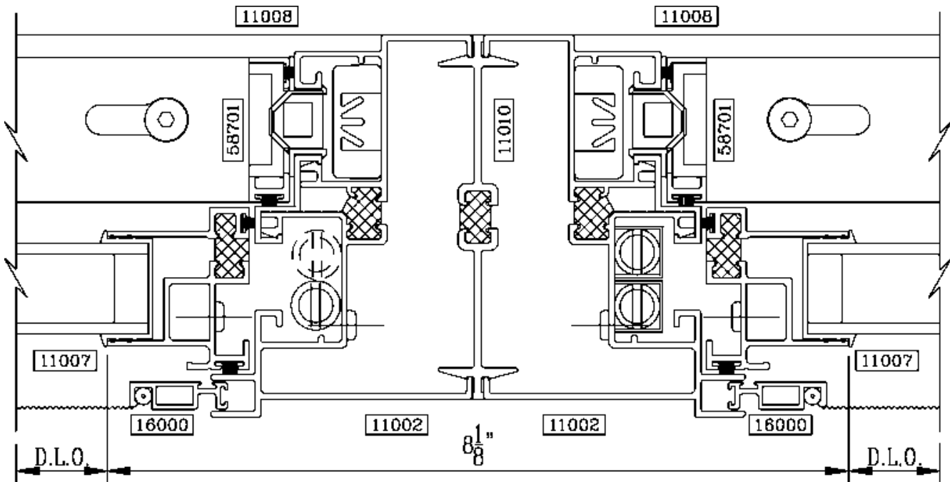
6 STACKING MULLION DOUBLE HUNG/DOUBLE HUNG
