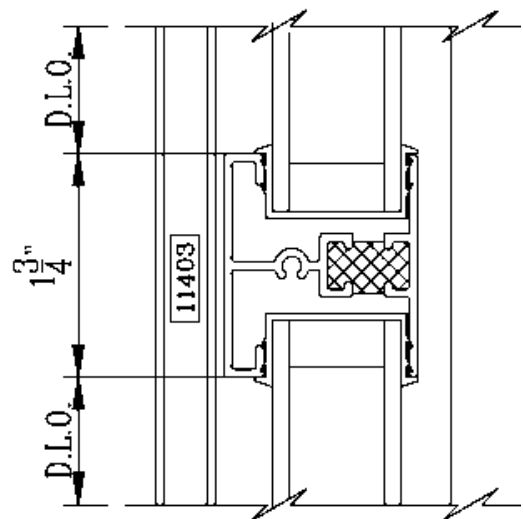
8 TRUE MUNTIN DOUBLE HUNG
