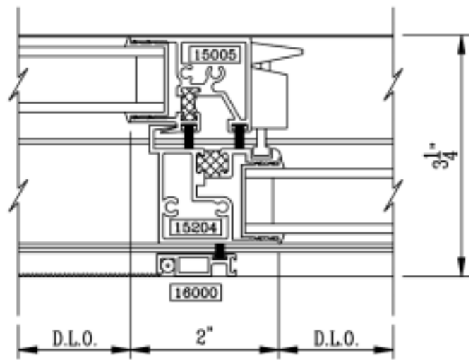
Meeting Rail Slider
