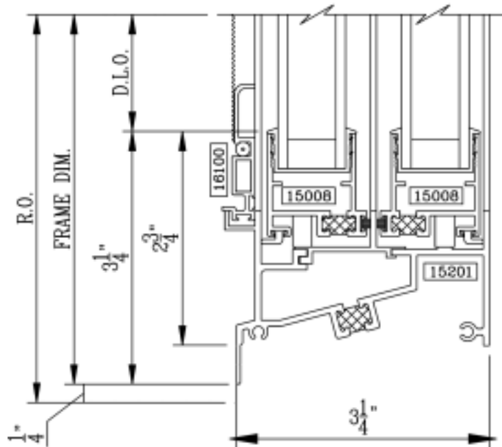
2 Sill Slider
