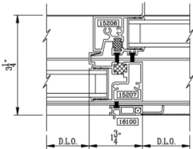
Reverse Interlock Meeting Rail Slider
