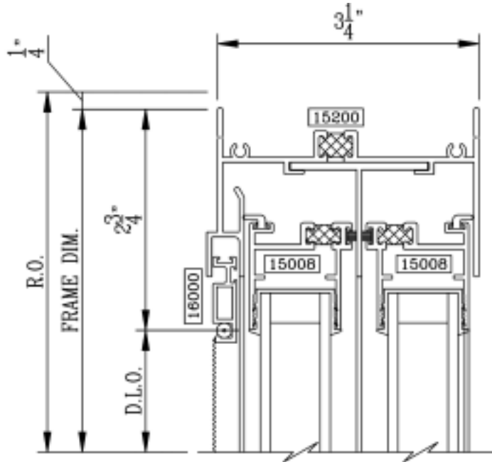
1 Head Slider
