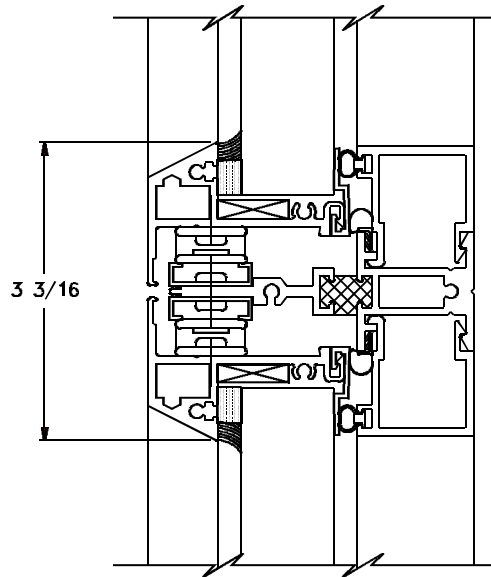
② INTEGRAL MULLION P7500
