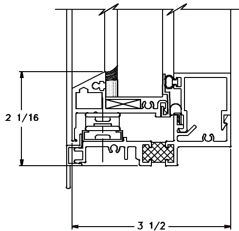
③ SILL P7500
