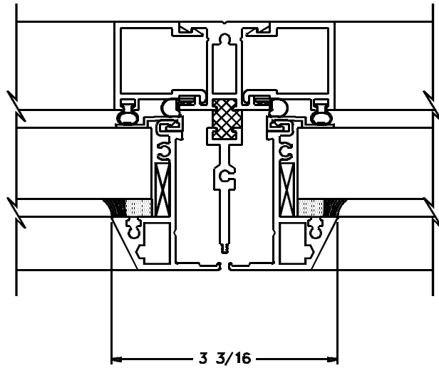
⑤ INTEGRAL MULLION P7500
